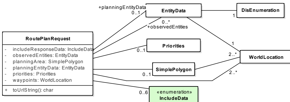
Figure 9: Description of the request to the route planning service. A request includes way points, data for the planning entity, and a bounding area for path planning. It also includes data for other relevant entities such as enemies within the planning area. IncludeData is an enumeration for what kind of additional data to include in the response, for example speed along the route.
