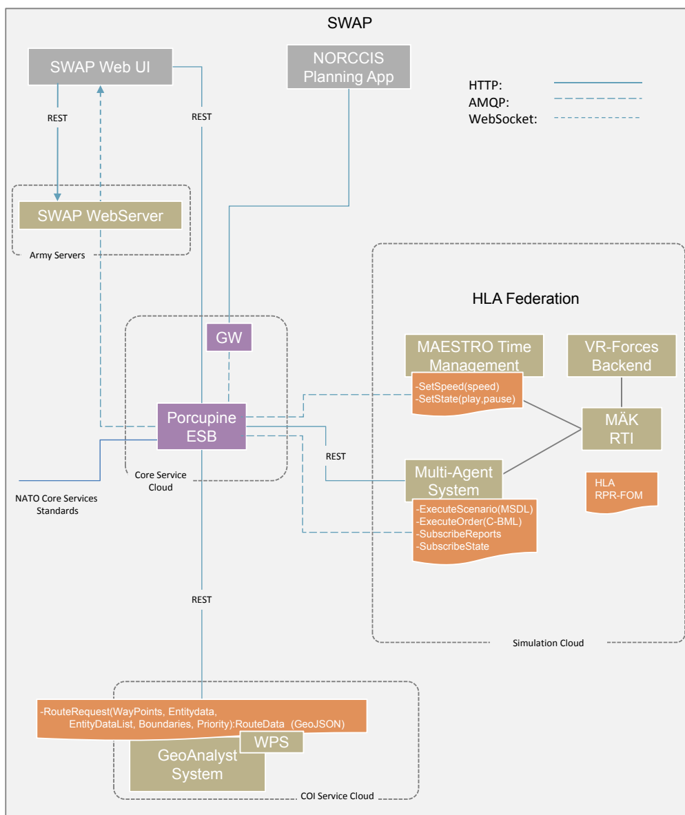
Figure 8: SWAP system architecture. Concrete systems (olive) with interfaces (orange) where applicable. Lines according to application layer protocols (HTTP, AMQP, WebSocket). Requests over lines to interfaces at provider. Responses over lines from interfaces to systems.
