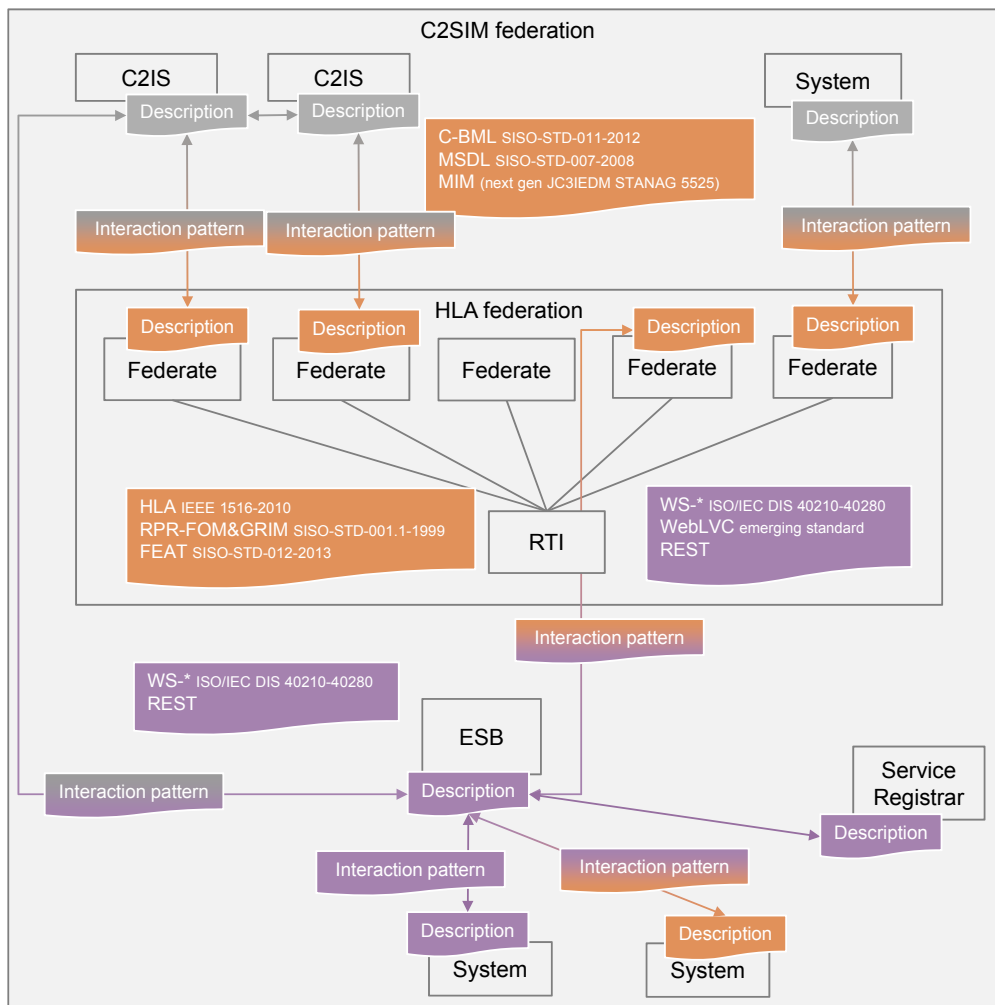
Figure 7: Reference Hybrid Architecture for C2SIM federation
